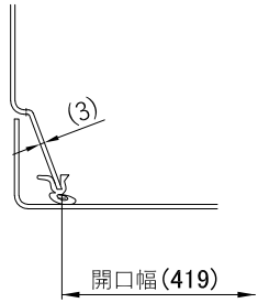
C-C断面概略図(FREE)
